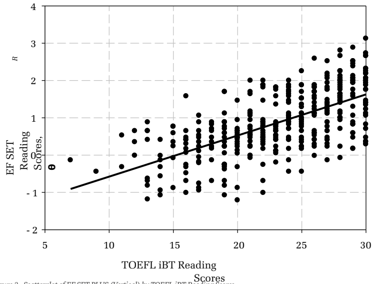
Figure 3. Scatterplot of EF SET PLUS (Vertical) by TOEFL iBT Reading Scores
