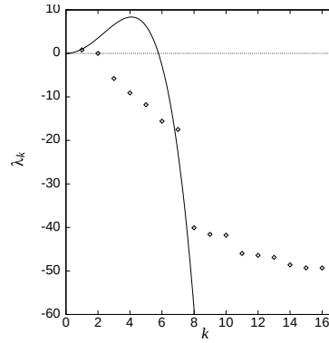
Figure 30.8: Floquet exponents \lambda_k (5.4) versus k for the least unstable spatio-temporally periodic orbit \bar{\Gamma} of the Kuramoto-Sivashinsky system, compared with the stability exponents (5.2) of the u(x, t) = 0 flat-front equilibrium, \lambda_k = k^2 - k^4 . The eigenvalues \lambda_k for k \geq 8 fall below the numerical accuracy of integration and are not meaningful. The cycle \bar{\Gamma} was computed using methods of chapter 16. System size \tilde{L} = 2.89109 , N = 16 Fourier modes truncation (from ref. [9]).
