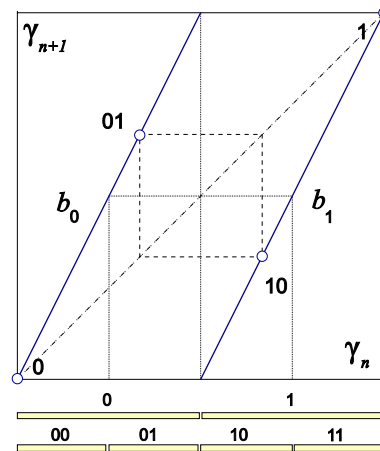
Figure 14.16: The n = 2 and 4 intervals state space partitions for the Bernoulli shift map (14.18), together with the fixed points \bar{0} , \bar{1} and the 2-cycle \bar{01} . For the doubling map (14.19) acting on the circle, \bar{0} is the only one fixed point, as x_1 = 1 = 0 \pmod{1} .
