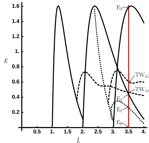
Figure 30.2: The energy (30.30) of the equilibria and relative equilibria that exist up to L = 22 , \tilde{L} = 3.5014 \dots , plotted as a function of the system size \tilde{L} = L/2\pi (additional equilibria, not present at L = 22 are given in ref. [21]). Solid curves denote 2- and 3-cell solutions E_2 and E_3 , dotted curves the GLMRT equilibrium E_1 , and dashed curves the relative equilibria TW_{\pm 1} and TW_{\pm 2} . The parameter \alpha of refs. [21, 27] is related to the system size by \tilde{L} = \sqrt{\alpha/4} .
