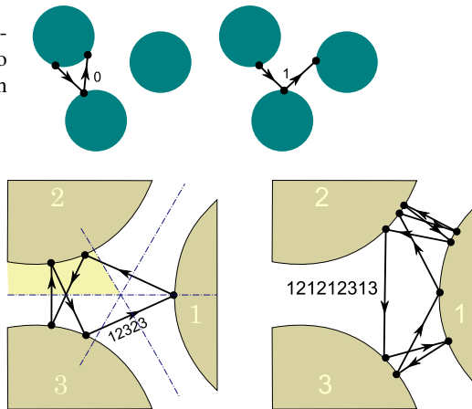
Figure 1.6: Binary labeling of the 3-disk pinball trajectories; a bounce in which the trajectory returns to the preceding disk is labeled 0, and a bounce which results in continuation to the third disk is labeled 1.
