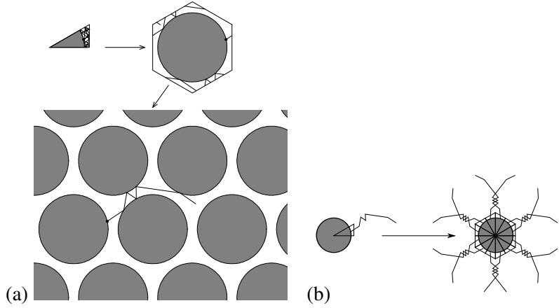
Figure 24.3: A periodic lattice of reflecting disks \hat{\mathcal{M}} is tiled by copies of the fundamental domain \tilde{\mathcal{M}} . (a) Motion in the fundamental domain \tilde{\mathcal{M}} (top left), the elementary cell \mathcal{M} (top right), and the full state space \hat{\mathcal{M}} (bottom). (b) The above trajectory unwrapped in the full space and its 11 copies obtained by applying the twelve D_6 point group actions to it. (from ref. [15]).
