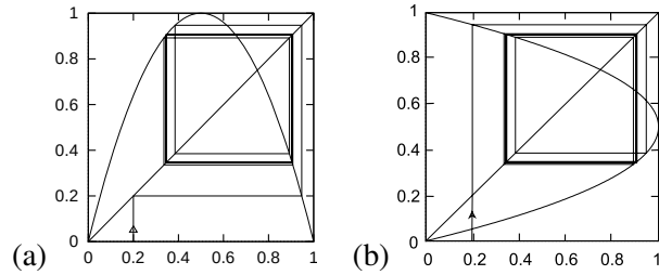
Figure 7.1: (a) The inverse time transient to the \overline{01} -cycle of the Ulam logistic map f(x) = 4x(1-x) from an initial guess x = 0.2 . (b) The same dynamics, but now plotted as the forward iteration of the doubly-valued inverse map f^{-1}(x) . At each iteration we chose the 0 (respectively 1) branch. For f(x) , the \overline{01} -cycle is an unstable cycle; for f^{-1}(x) it is a stable, attracting cycle.
