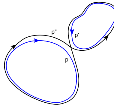
Figure 1.11: A longer cycle p'' shadowed by a pair (a 'pseudo orbit') of shorter cycles p and p' .
