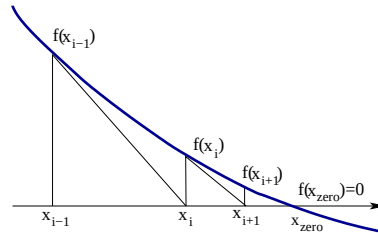
Figure 7.3: Newton's method for finding zeros of functions, f(x_{\text{zero}}) = 0 , an idealized sketch.
