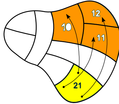
Figure 17.1: Points from region \mathcal{M}_{21} reach regions \{\mathcal{M}_{10}, \mathcal{M}_{11}, \mathcal{M}_{12}\} in one time step. Labeling exemplifies the ‘shift map’ of example 14.5 and (14.12).
