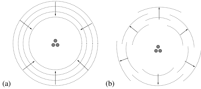
Figure 40.1: (a) Incoming spherical waves running into an obstacle. (b) Superposition of outgoing spherical waves scattered from an obstacle.
