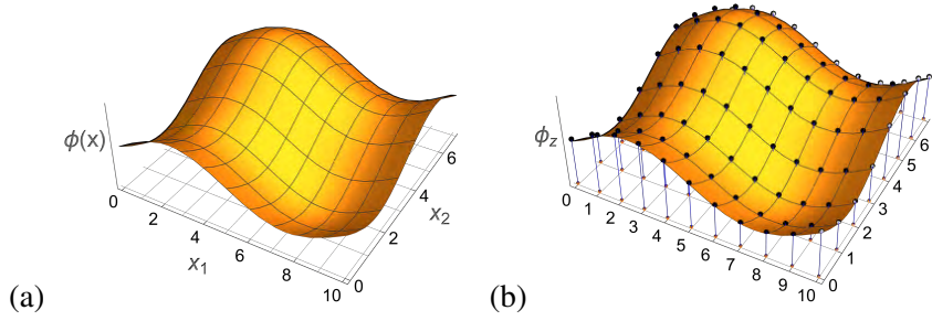
Figure A24.1: Discretization of a field over two-dimensional spacetime. (a) A periodic scalar field configuration \phi(x) over a primitive cell of spatial period L , temporal period T , plotted as a function of continuous coordinates x \in \mathbb{R}^2 . (b) The corresponding discretized field configuration (A24.13) over [10 \times 7]_0 primitive cell, with the field value \phi_z at the lattice site z \in \mathbb{Z}^2 indicated by a dot. (Han Liang [10].)
