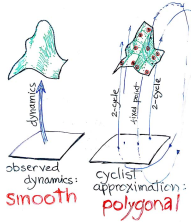
Figure 15.13: Reduction of a continuous-time flow (left frame) to a set of return maps (right frame), with a point on 1-cycle and the two cycle points of a 2-cycle used as template points.
