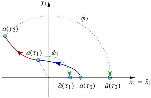
Figure 13.3: Method of moving frames for the two-modes flow \text{SO}(2) -equivariant under (12.42), with slice through \hat{a}' = (1, 0, 0, 0) , group tangent t' = (0, 1, 0, 0) . The equivariant flow is 4-dimensional: shown is the projection on the (x_1, y_1) plane. The clockwise orientation condition restricts the slice to the 3-dimensional half-hyperplane \hat{x}_1 > 0, \hat{y}_1 = 0 . A trajectory started on the slice at a(\tau_0) = \hat{a}(\tau_0) , evolves to a state space point with a non-zero y_1(\tau_n) . To bring this point back to the slice, compute the polar angle \phi_n of a(\tau_n) in the (x_1, y_1) plane. Rotate a(\tau_n) clockwise by \phi_n to \hat{a}(\tau_n) = g(-\phi_n)a(\tau_n) , so that the equivalent point on the circle lies on the slice, \hat{y}_1(\tau_n) = 0 . See sect. 13.5.
