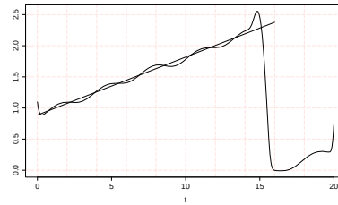
Figure 6.3: A numerical computation of the logarithm of the stretch \hat{n}^\top (J'^\top J') \hat{n} in formula (6.10) for the Rössler flow (2.30), plotted as a function of the Rössler time units. The slope is the leading Lyapunov exponent \lambda \approx 0.09 . The exponent is positive, so numerics lends credence to the hypothesis that the Rössler attractor is chaotic. The big unexplained jump illustrates perils of Lyapunov exponents numerics. (J. Mathiesen)
