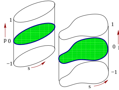
Figure 9.3: In D = 2 , the billiard Poincaré section is a cylinder, where the parallel momentum p ranges over p \in \{-1, 1\} and the s coordinate is cyclic along each connected component of \partial Q . The rectangular figure 9.2(b) is an unfolded cylinder, with periodic boundary conditions gluing together the left and right edge of the rectangle.
