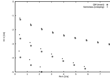
Figure 41.3: The shape resonances of the 1-disk system in the complex k plane in units of the disk radius a . The boxes label the exact quantum mechanical resonances (given by the zeros of H_m^{(1)}(ka) for m = 0, 1, 2 ), the crosses label the diffractive semiclassical resonances (given by the zeros of the creeping formula in the Airy approximation (41.36) up to the order O([ka]^{1/3}) ).
