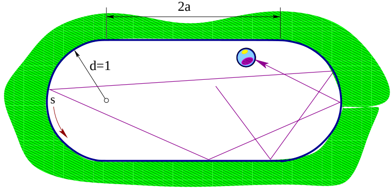
Figure 9.1: The stadium billiard is a 2-dimensional domain bounded by two semi-circles of radius d = 1 connected by two straight walls of length 2a . At the points where the straight walls meet the semi-circles, the curvature of the border changes discontinuously; these are the only singular points of the flow. The length a is the only parameter.
