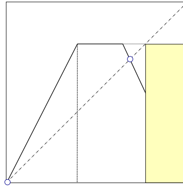
Figure 14.11: The dike map is obtained by slicing off the top portion of the tent map in figure 14.9(a). Any full tent map orbit that visits the primary pruning interval (\kappa, 1] is inadmissible. The admissible orbits form the Cantor set obtained by removing from the unit interval the primary pruning interval and all its iterates. Any admissible orbit has the same topological coordinate and itinerary as the corresponding full tent map orbit.
