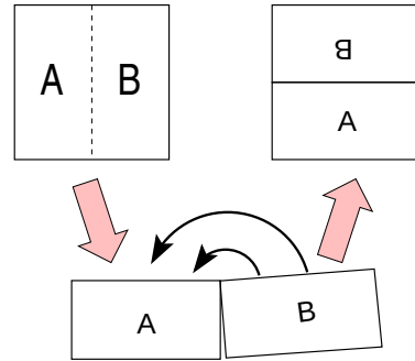
Figure 15.6: The orientations involved with kneading a Danish pastry mimics the horseshoe dynamics of figure 15.5 by (1) squashing the unit square by factor 1/2, (2) stretching it by factor 2, and (3) folding the right half back over the left half.
