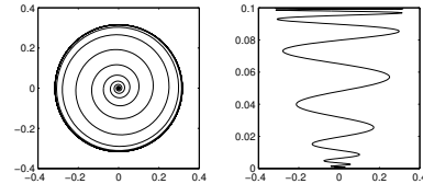
Figure 31.2: State trajectory starting close to x_q = 0 and with \mu = 1/10 for the system (31.28) in x, y -plane (left) and the (x, z) -plane (right).
