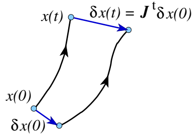
Figure 1.9: The Jacobian matrix J^t maps an infinitesimal displacement \delta x at x_0 into a displacement J^t(x_0)\delta x a finite time t later.
