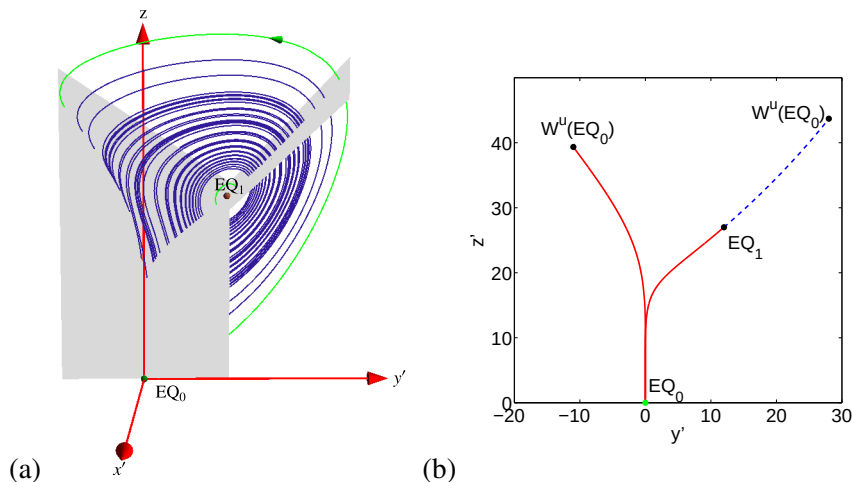
Figure 14.14: (a) A Poincaré section of the Lorenz flow in the doubled-polar angle representation, figure 11.2 (b), given by the [y', z] plane that contains the z -axis and the equilibrium EQ_1 . Most of the section plane except for the two shaded trapezoids is removed to aid visualization of the flow. x' axis points toward the viewer. (b) The Poincaré section plane. Crossings into the section are marked red (solid) and crossings out of the section are marked blue (dashed). Outermost points of both in- and out-sections are given by the EQ_0 unstable manifold W^u(EQ_0) intersections. (E. Siminos)
