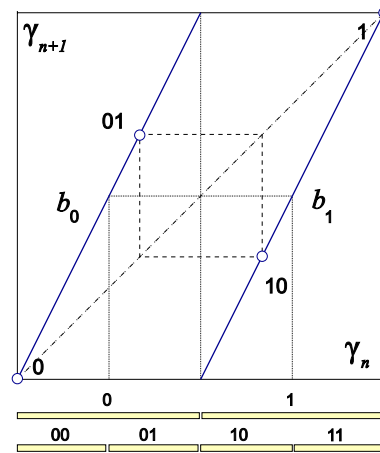
Figure 14.8: The n = 2 and 4 intervals state space partitions for the Bernoulli shift map (14.18), together with the fixed points \bar{0} , \bar{1} and the 2-cycle \bar{01} .
