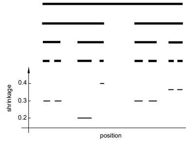
Figure A33.1: Construction of the steps of the scaling function from a Cantor set. From one level to the next in the construction of the Cantor set, each parent segment changes into two children segments. The shrinkage of the last level of the construction is plotted and by removing the gaps one has an approximation to the scaling function of the Cantor set.
