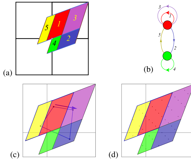
Figure 18.4: (Continued from figure 14.18) (a) The sub-rectangles M_i of figure 14.18(c). (b) Admissible orbits correspond to walks on the transition graph of figure 14.18(d), with rectangles M_A (red) and M_B (green) as nodes, and the links labeled by 5-letter alphabet (18.42), see the loop expansion (18.43). (c) The \overline{0111} is an example of a period-4 prime cycle. (d) All prime period-4 periodic points, see the periodic points, one-per prime orbit (18.50). Note that they all land in the partition (a).
