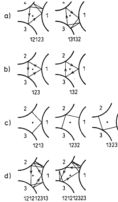
Figure 15.14: Some examples of 3-disk cycles: (a) \overline{12123} and \overline{13132} are mapped into each other by the flip across 1 axis. Similarly, (b) \overline{123} and \overline{132} are related by flips, and (c) \overline{1213} , \overline{1232} and \overline{1323} by rotations. (d) The cycles \overline{121212313} and \overline{121212323} are related by rotation and time reversal. These symmetries are discussed in chapter 11 (from ref. [15]).
