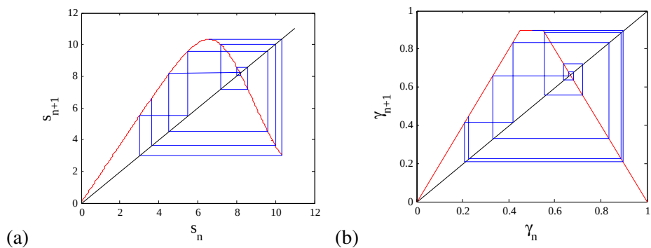
Figure 14.13: (a) Web diagram generated by the trajectory of the critical point, the unimodal Rössler return map of figure 14.7 (b). (b) The web diagram for the corresponding ‘canonical’ dike map (14.6) with the same kneading sequence. (A. Basu and J. Newman)
