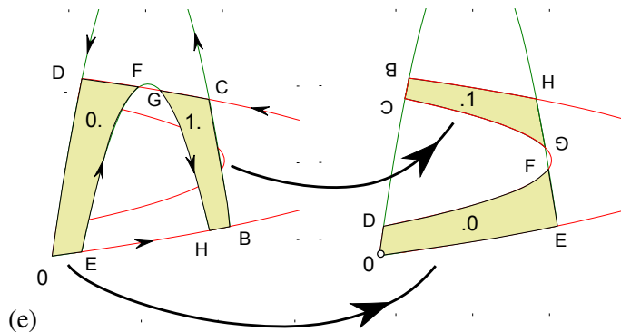
Figure 15.5: The dynamics maps two (past) strips \mathcal{M}_0, \mathcal{M}_1 into two (future) strips \mathcal{M}_0, \mathcal{M}_1 . The corners are labeled to aid visualization. Note that the BCGH strip is rotated by 180 degrees. (P. Cvitanović and Y. Matsuoka)
