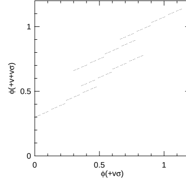
Figure A33.3: The spin adding map F_+ for the potential J(n) = \sum n^2 a^n . The action of the map takes the value of the interaction energy between + and the semi-infinite configuration \{\sigma_1, \sigma_2, \sigma_3, \dots\} and returns the interaction energy between + and the configuration \{+, \sigma_1, \sigma_2, \sigma_3, \dots\} .
