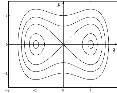
Figure 8.1: Phase plane of the unforced, undamped Duffing oscillator. The trajectories lie on level sets of the Hamiltonian (8.30).
