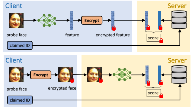
Figure 1. Secure FR systems. (1) Top: existing secure FR system which encrypts only the features, rather than raw face images, limits practical utility and security; (2) bottom: proposed end-to-end encrypted face recognition system which ensures stronger protection of the user’s face image and feature while safeguarding the server’s reference database.
