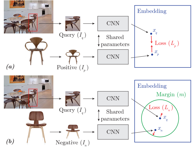
Figure 9: Training procedure. In each mini-batch, we include a mix of (a) positive and (b) negative examples. In each iteration, we take a step to decrease the loss function; this can be viewed as “forces” on the points (red arrows). Photo credit: Austin Rooke.
