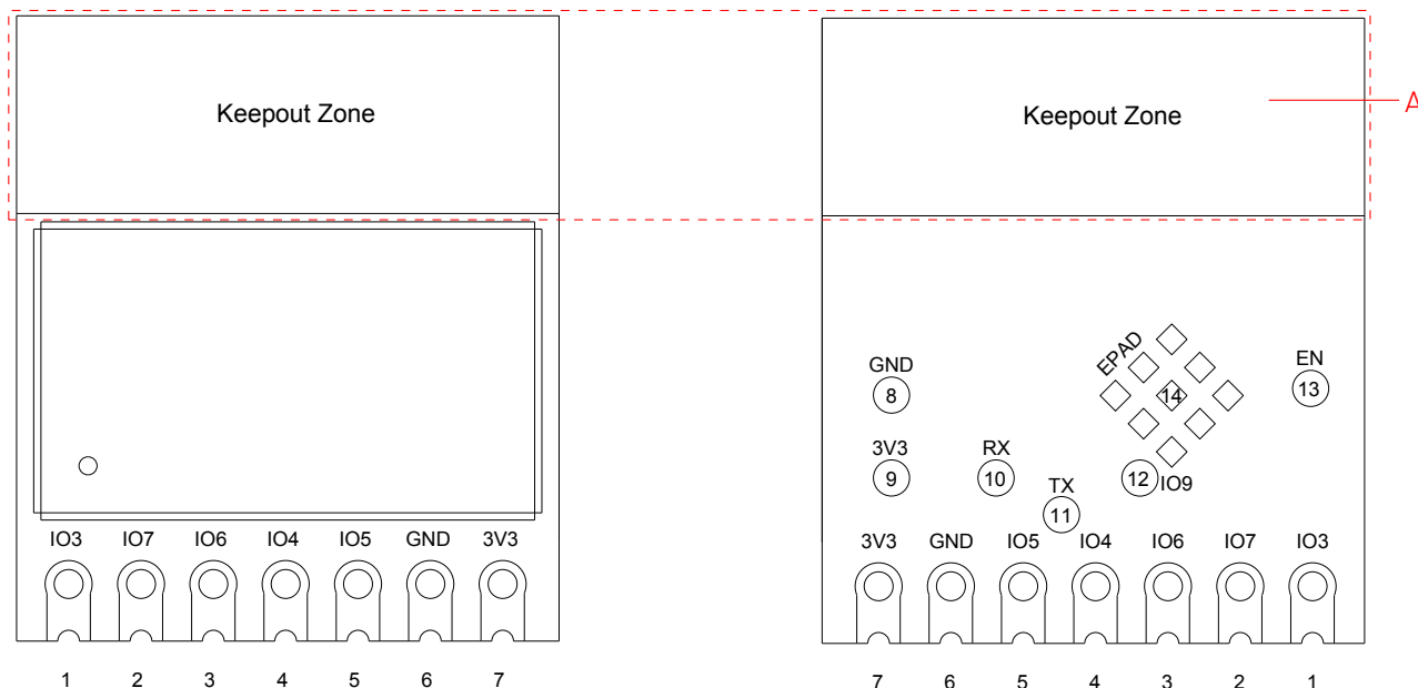
Figure 3-1. Pin Layout (Top View and Bottom View)
