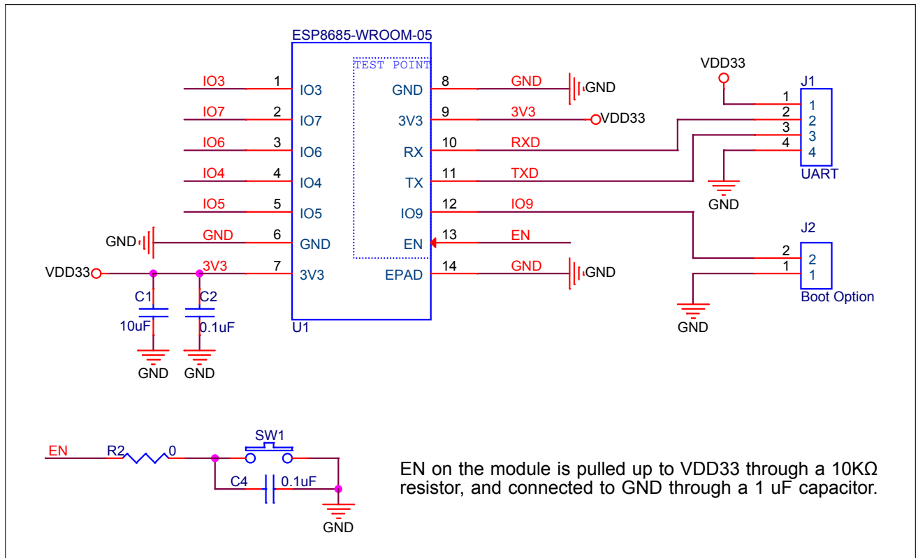
Figure 9-1. Peripheral Schematics
