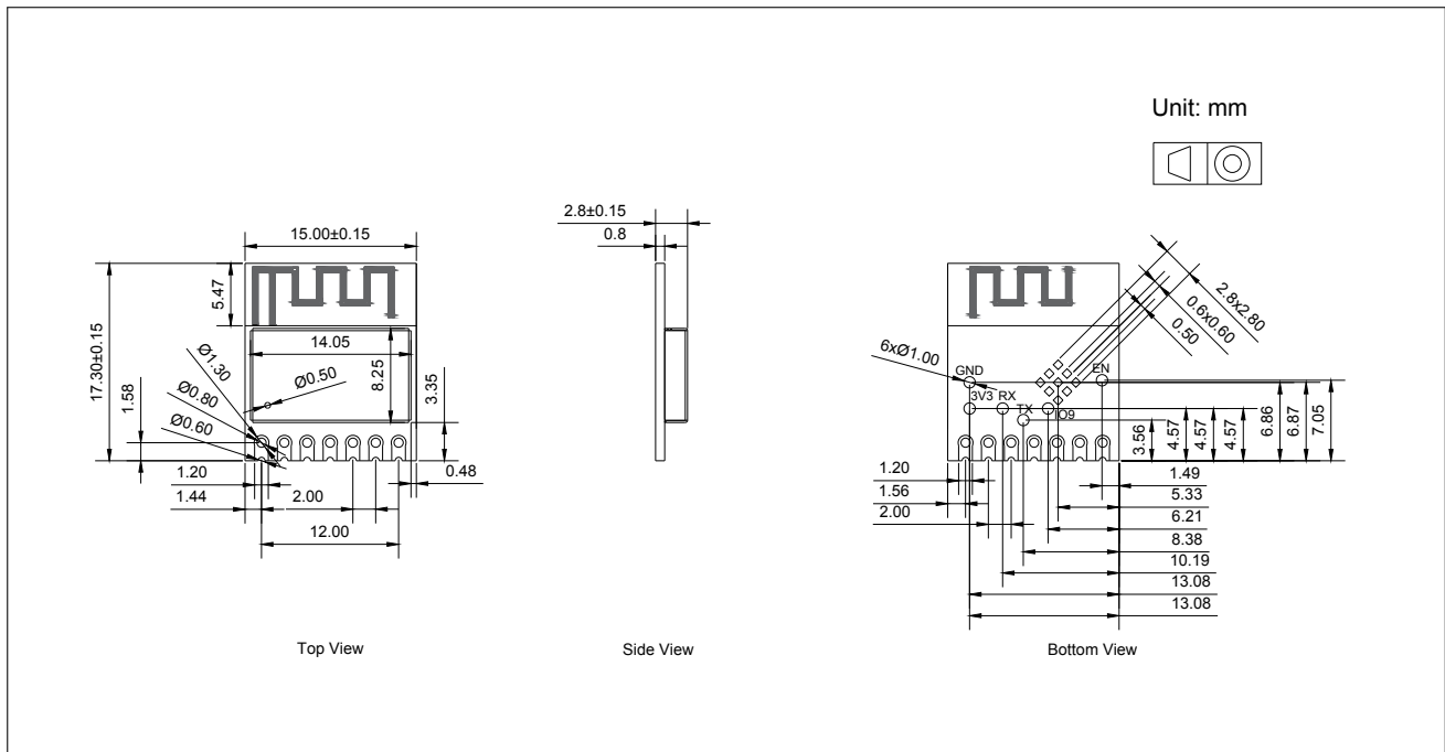
Figure 10-1. Physical Dimensions
