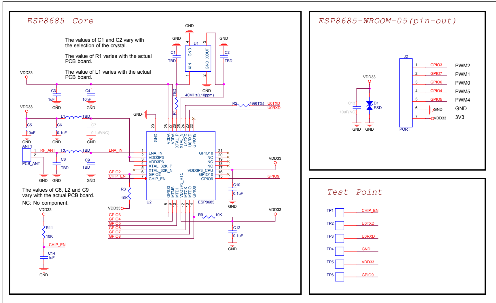
Figure 8-1. Schematics
