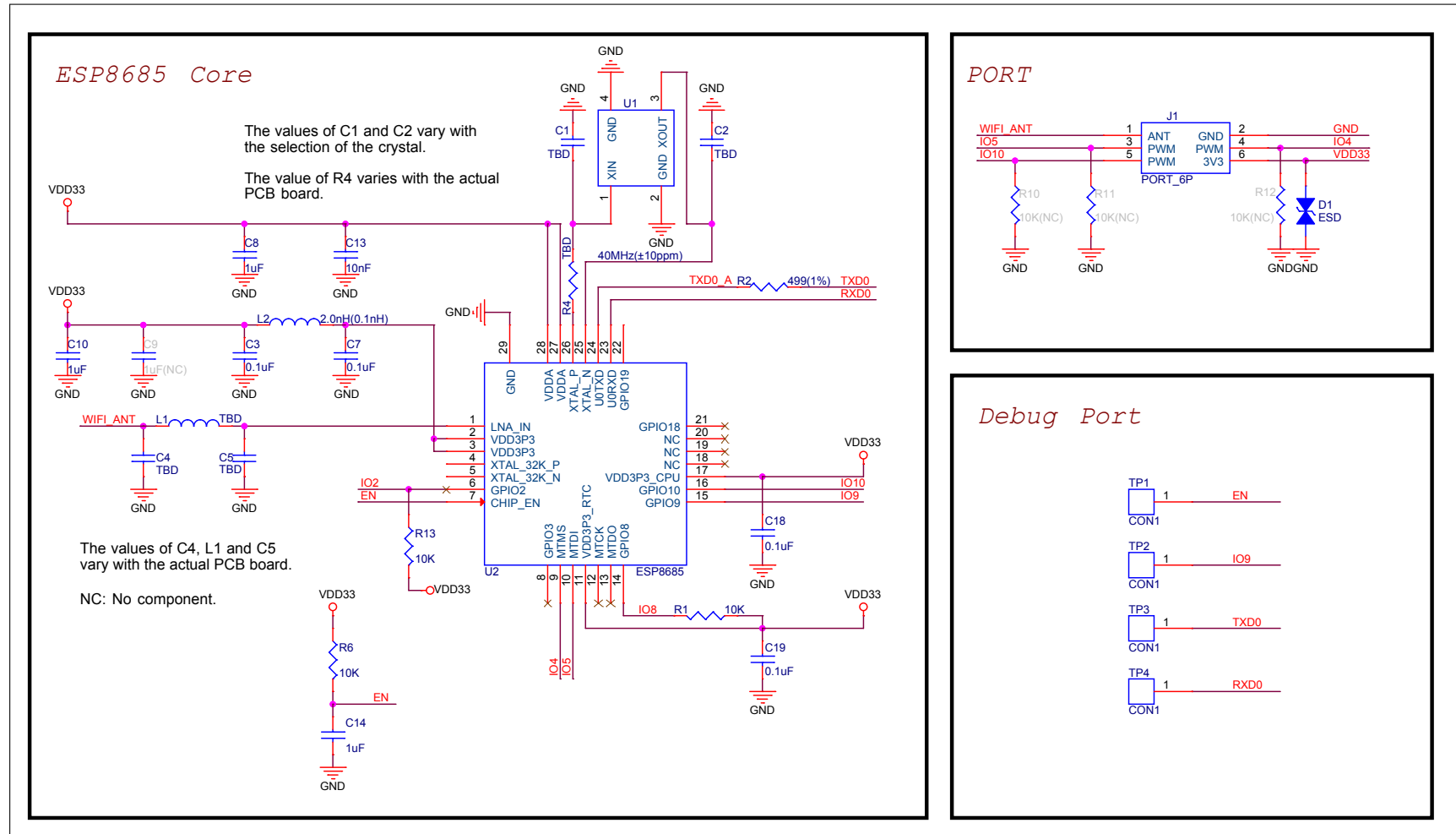
Figure 8-1. Schematics
