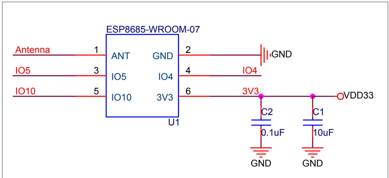
Figure 9-1. Peripheral Schematics
