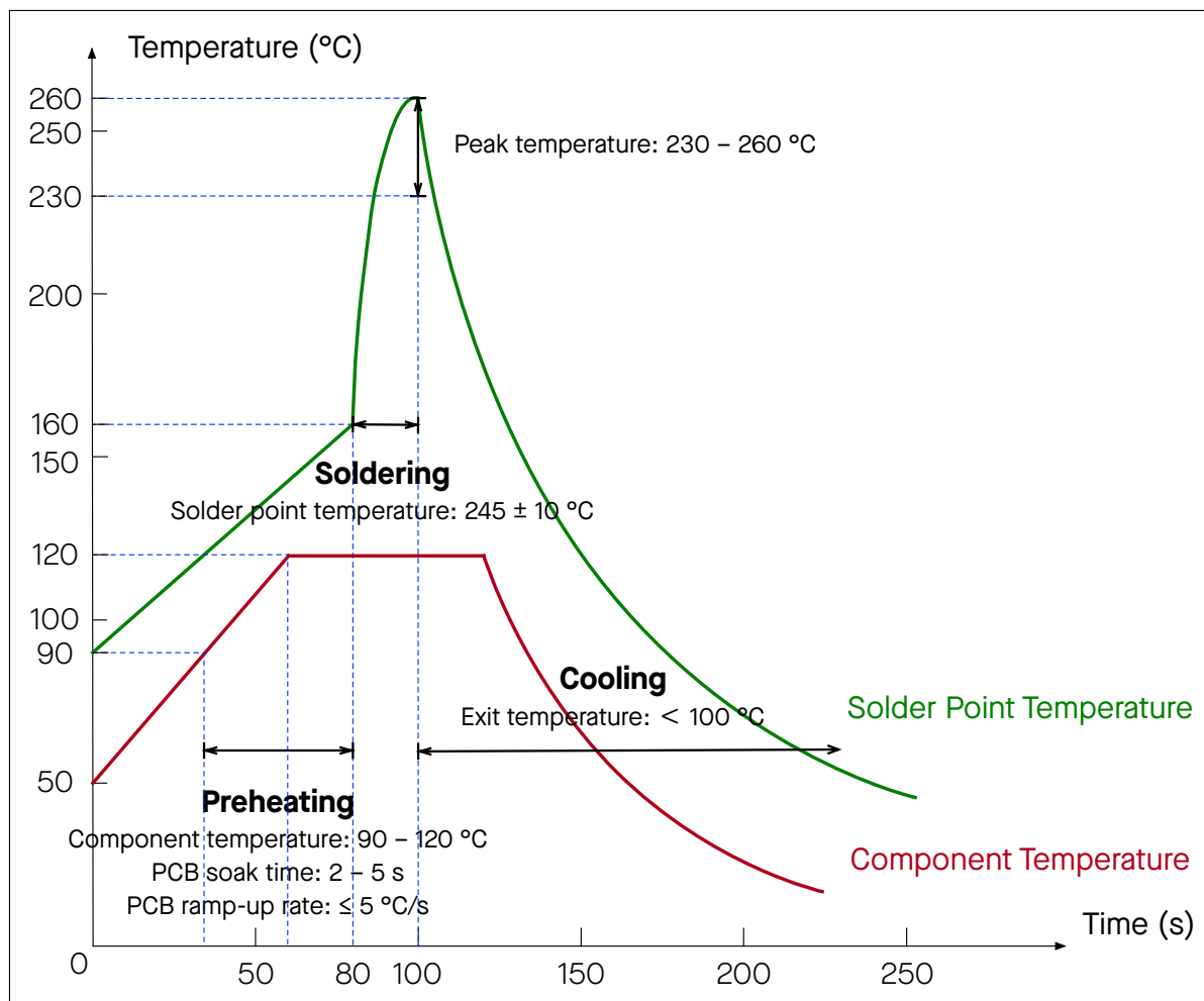
Figure 12-1. Wave Soldering Profile
